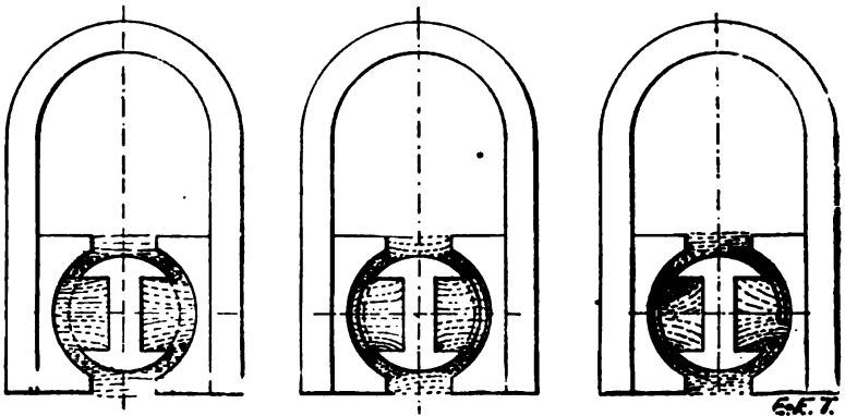
FIG. 341.—Diagram of the Construction and Operation of the Sims-Bosch Igniting Magneto. In this machine the armature is stationary, the lines being cut by an open sleeve rotating between it and the field pieces. The first diagram shows the convergence of the lines of force before the rotating sleeve has been inserted; the second shows the lines when the sleeve is directly across the magnetic lines; the third, where the sleeve is in position at oblique angles to the lines. As may be understood, this arrangement produces a very powerful variation of the field and a very strong output of E. M. F.
